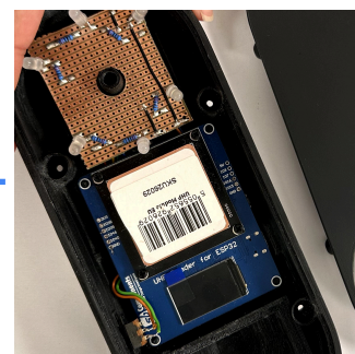
Lay UHF RFID Reader and push PCB into snap fits
